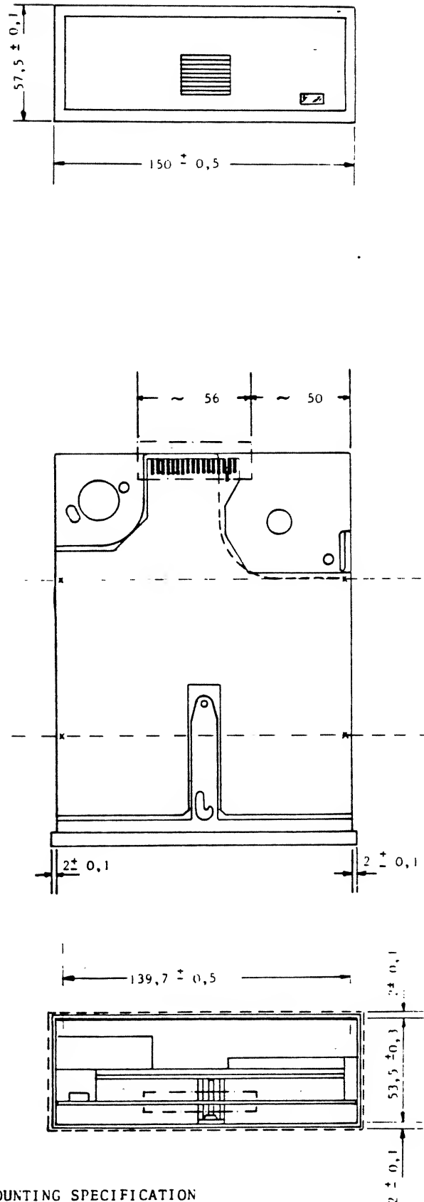
FIGURE 3 - 10. MOUNTING SPECIFICATION
