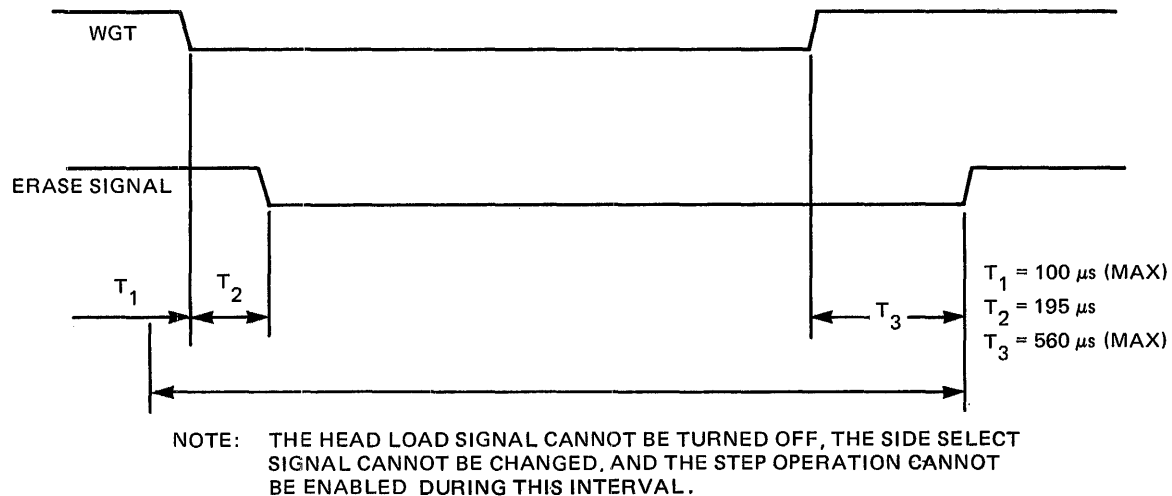
Figure 3-4 WGT Timing
