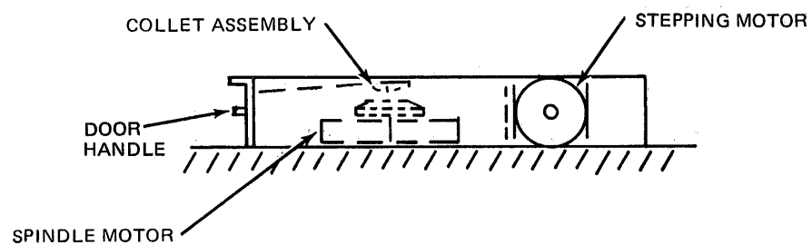
Figure 2-4 Horizontal Installation
