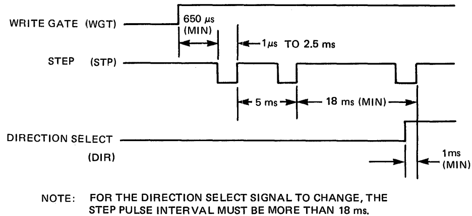
Figure 3-11 Access Timing
