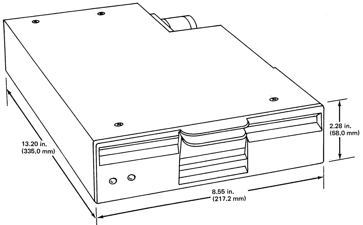
Figure 2-2 Model FD1165 Physical Dimensions
