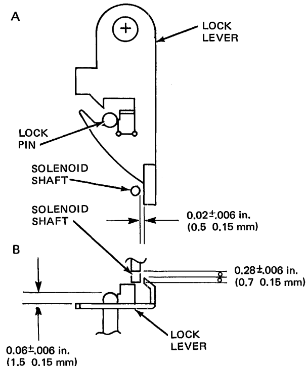
Figure 4-20 Adjusting the Door Lock Solenoid
