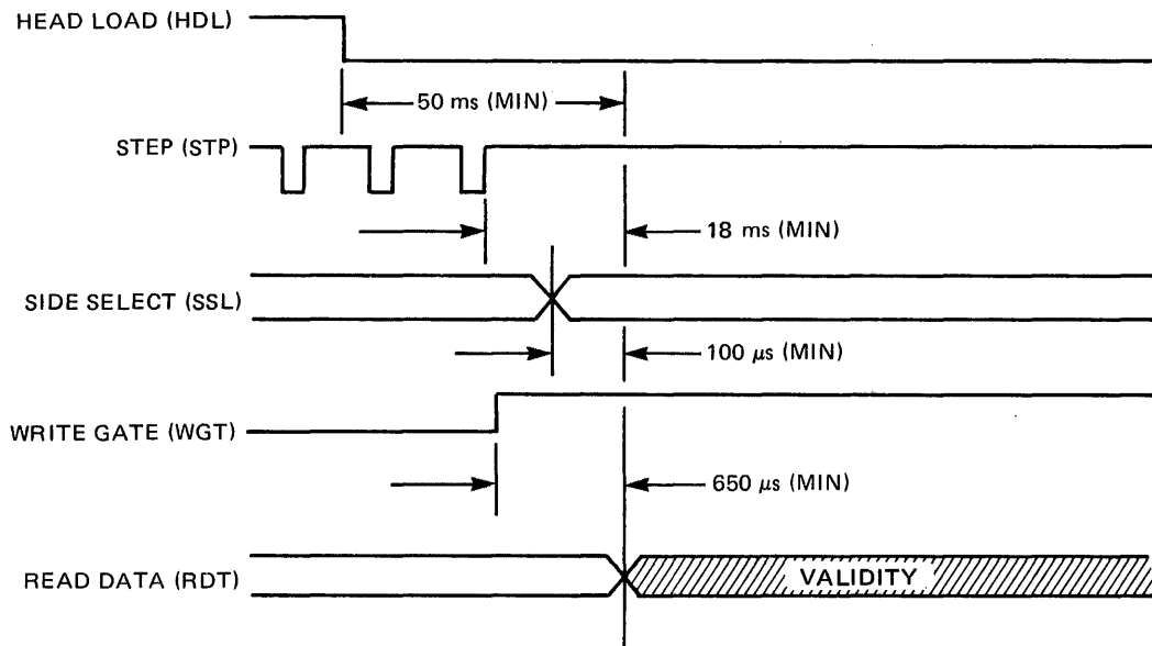
Figure 3-13 Read Timing
