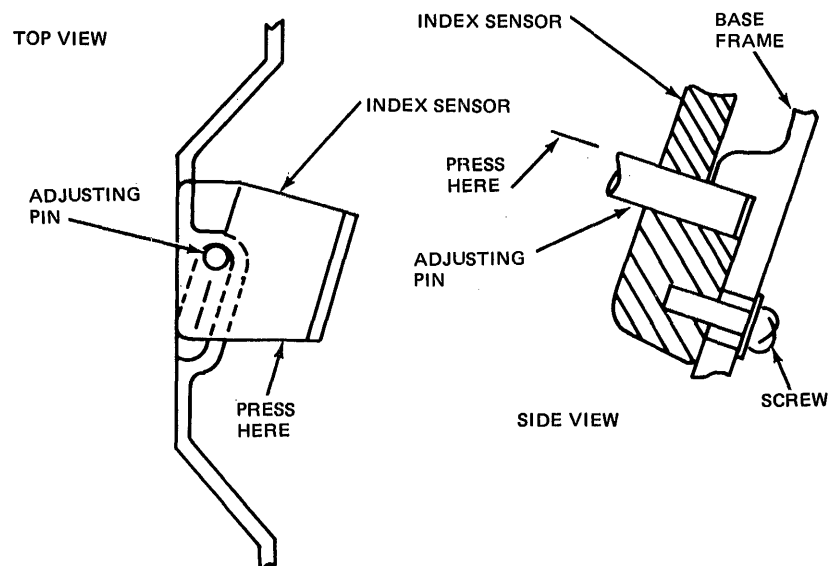
Figure 4-12 Installing the Index Sensor
