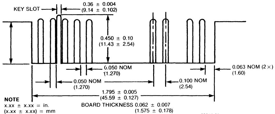
FIGURE 3-2. J1 CONNECTOR DIMENSIONS
