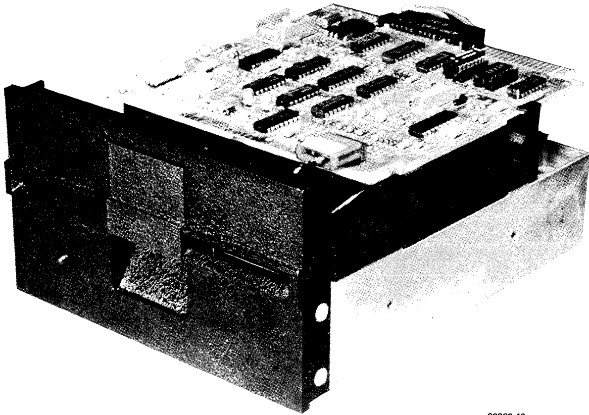
FIGURE 1-1. SA400L MINIFLOPPY™ DISKETTE DRIVE
