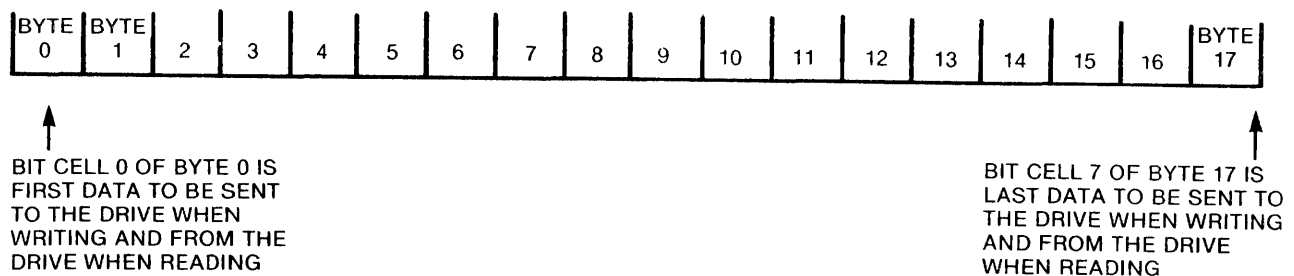
FIGURE 6-2. DATA BYTES
