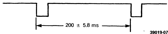
FIGURE 2-3. INDEX TIMING (SA104 MEDIA)
