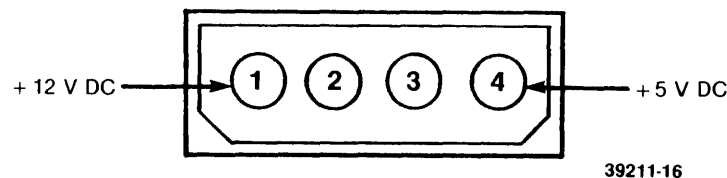
FIGURE 3-3. J2 CONNECTOR
