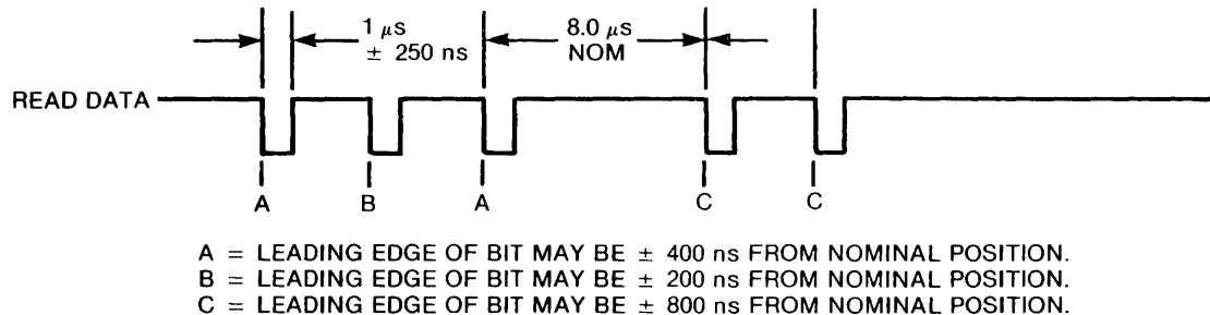
FIGURE 1-5. READ SIGNAL TIMING
