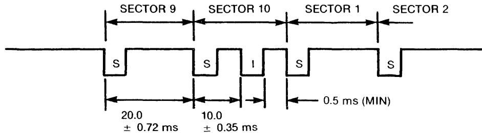
FIGURE 2-4. INDEX/SECTOR TIMING (SA105/107 MEDIA)
