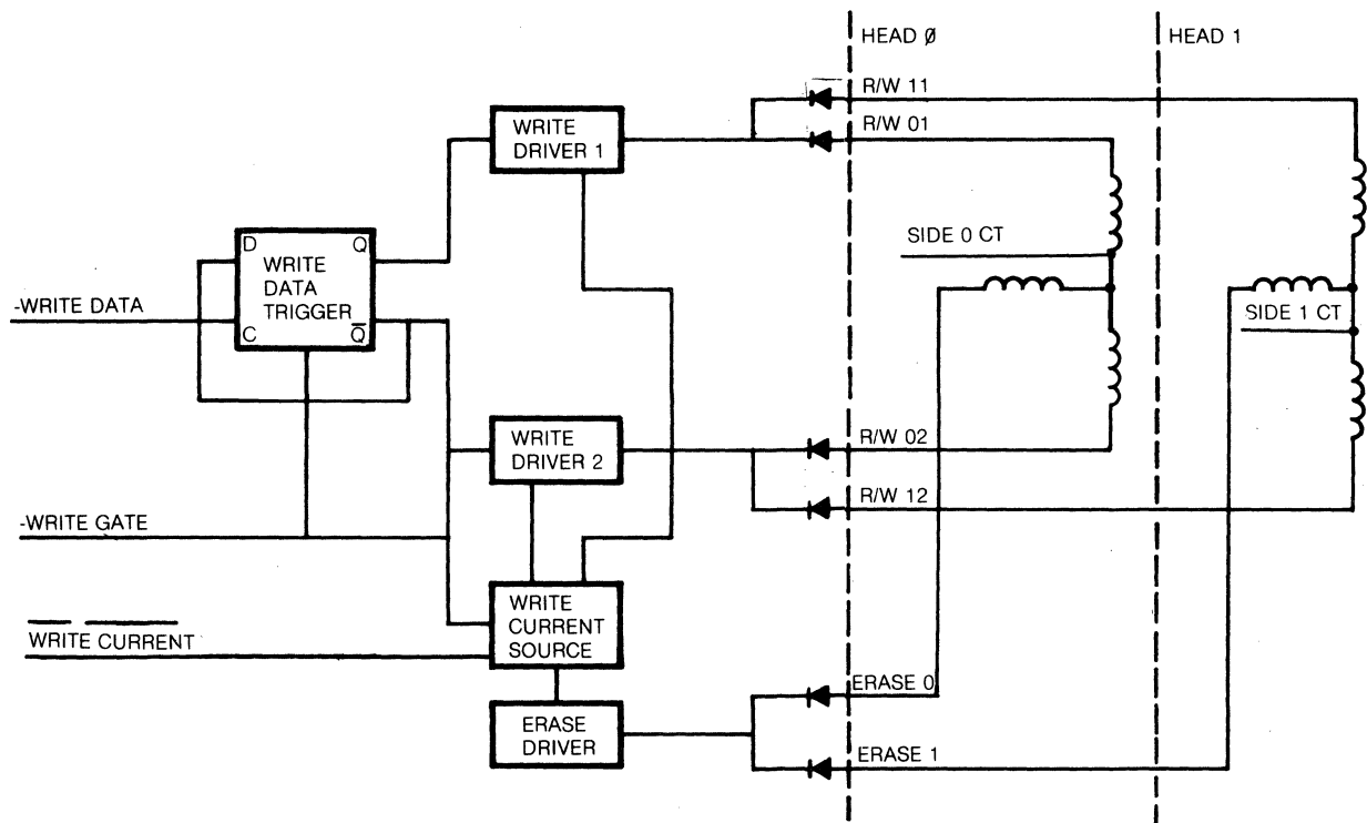
FIGURE 31. WRITE CIRCUIT FUNCTIONAL DIAGRAM
