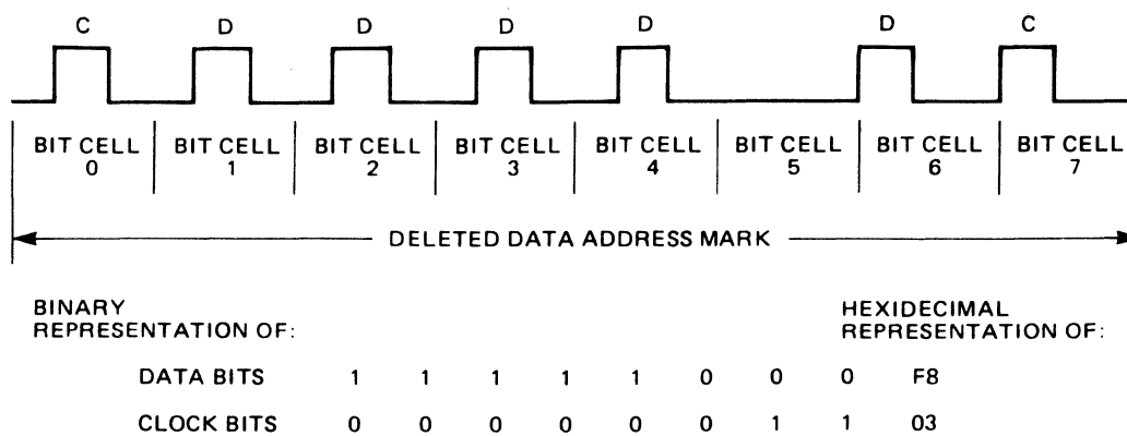
FIGURE 17. MFM DELETED DATA ADDRESS MARK
