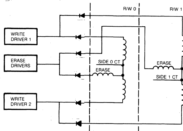
FIGURE 30. READ/WRITE HEADS
