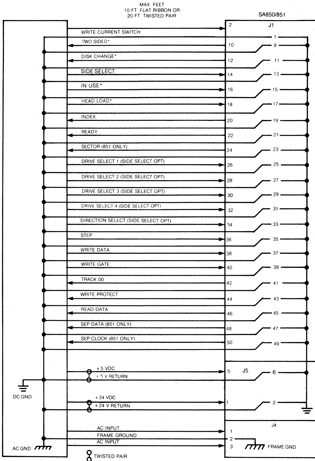
FIGURE 34. INTERFACE CONNECTIONS
