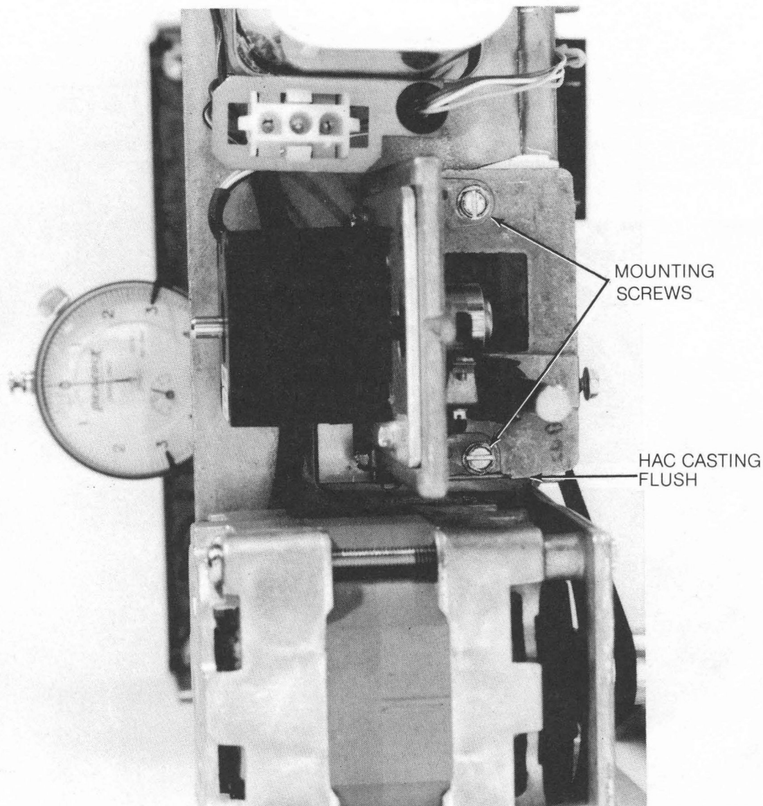
FIGURE 44. PENETRATION ADJUSTMENT
