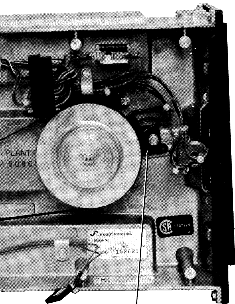
INDEX/SECTOR PHOTO TRANSISTOR
