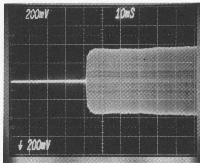
FIGURE 37. HEAD LOAD TIMING
