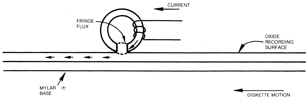
FIGURE 26. BASIC READ/WRITE HEAD
