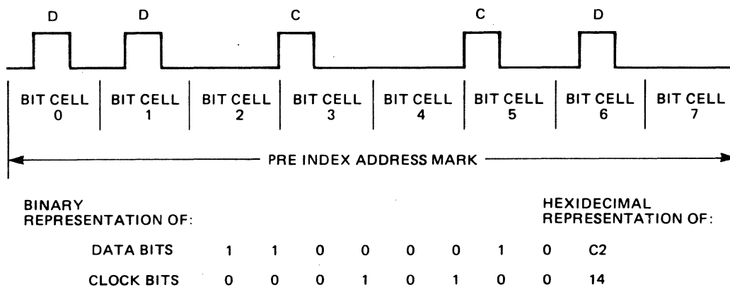
FIGURE 18. MFM INDEX PRE ADDRESS MARK
