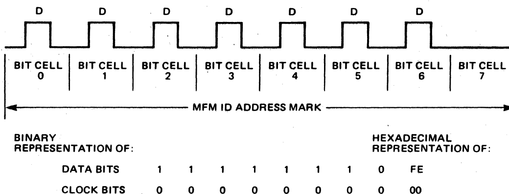
FIGURE 15. MFM ID ADDRESS MARK
