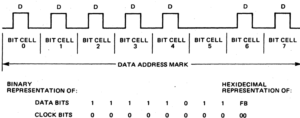
FIGURE 16. MFM DATA ADDRESS MARK
