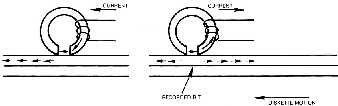
FIGURE 27. RECORDED BIT
