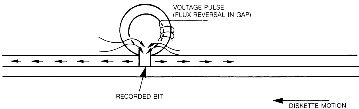
FIGURE 28. READING A BIT
