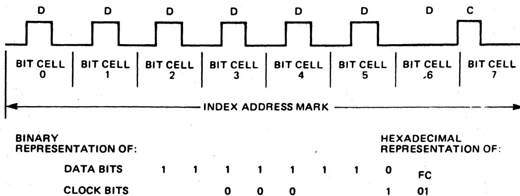
FIGURE 14. MFM INDEX ADDRESS MARK
