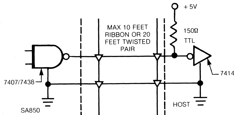
FIGURE 35. INTERFACE SIGNAL DRIVER/RECEIVER
