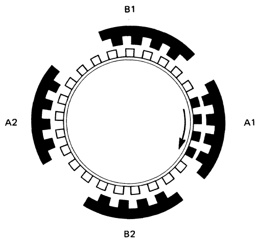
FIGURE 21. COUNT 0
