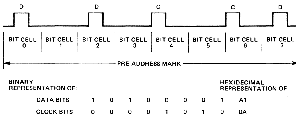
FIGURE 19. MFM PRE ID/DATA ADDRESS MARK
