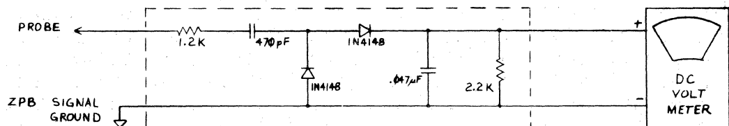
FIGURE 1C: A.C. SIGNAL DETECTOR
